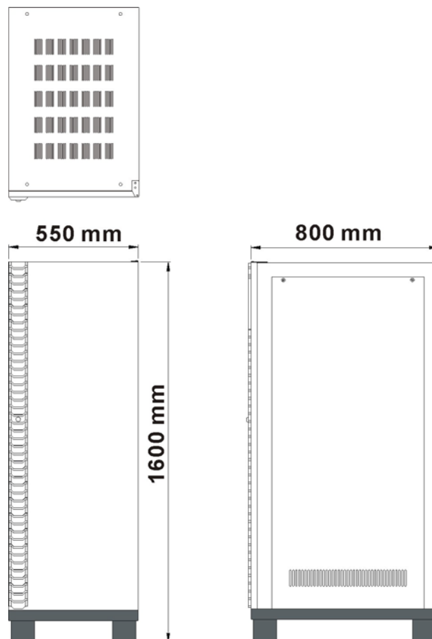
BATTERY CABINET
