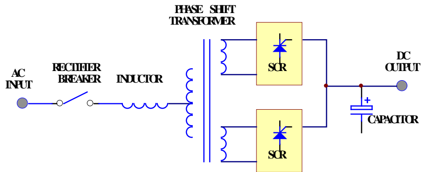
12-PULSE FULL CONTROL RECTIFIER
