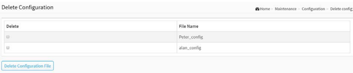
Figure 17-1.5: Delete Configuration
