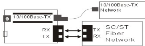
Figure 1 Schematic drawing of connection
